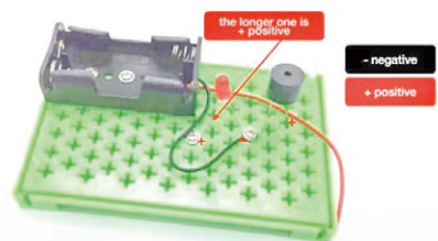
Step 2: Connect the LED light and the buzzer
